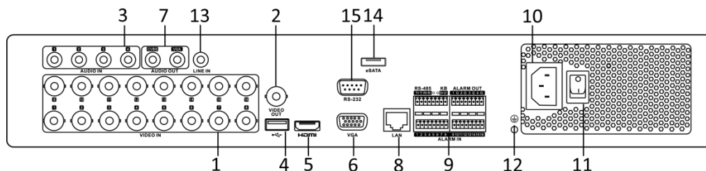
Figure 1. 14 Rear Panel of DS-7300HQHI-F4/N
