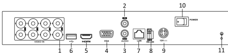
Figure 1. 10 Rear Panel of DS-7200HGHI-E1/E2
