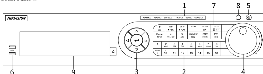
Figure 1. 5 Front Panel of DS-8100HQHI-F/N
