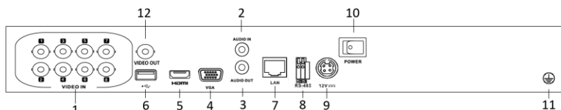
Figure 1. 12 Rear Panel of DS-7200HQHI-F2/N
